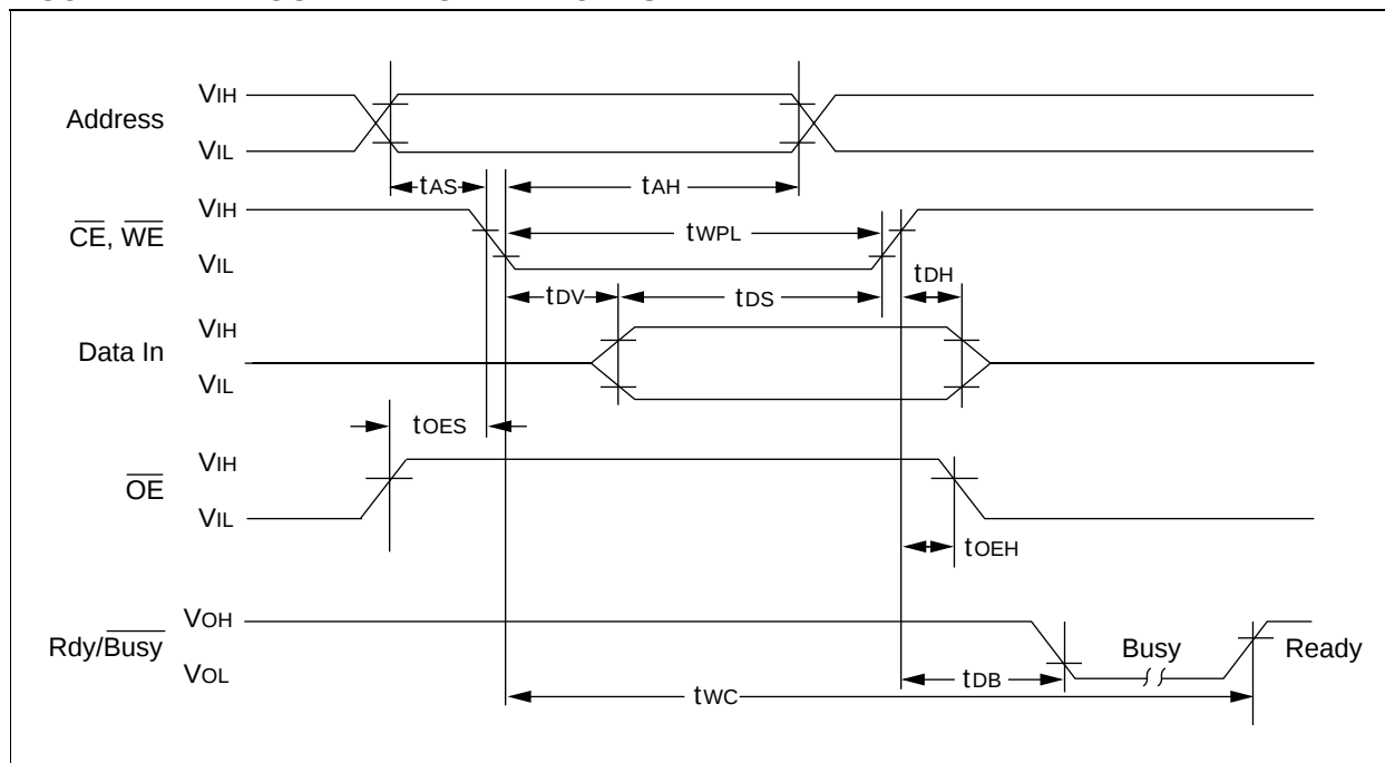
FIGURE 1-2: PROGRAMMING WAVEFORMS
